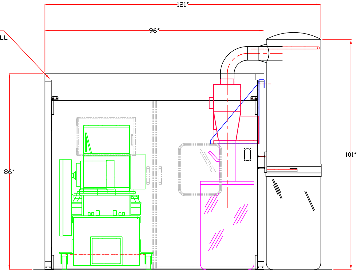
MODEL 22 DISINTEGRATOR
