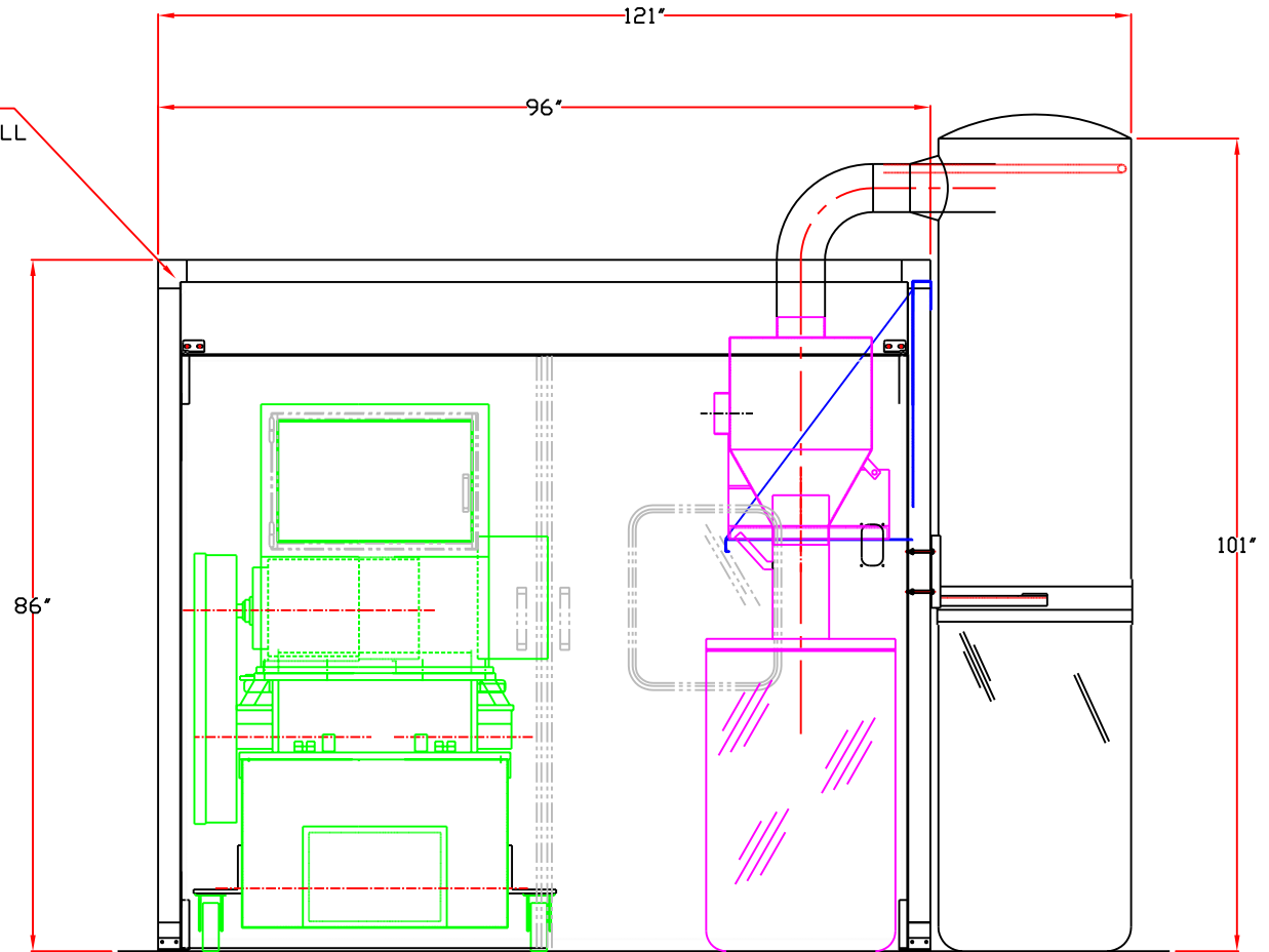
MODEL 23/5 DISINTEGRATOR
